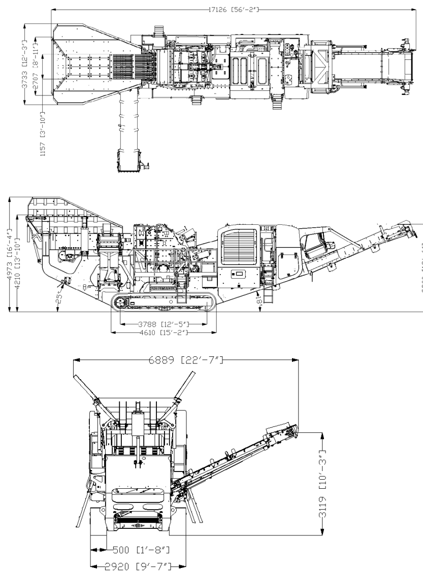
Figure 4: Trakpactor 550 - VGF, Standard Product Conveyor Working Position
