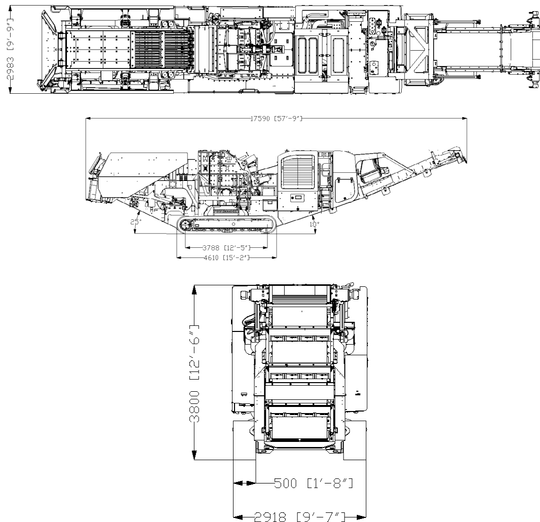
Figure 5: Trakpactor 550 - VGF, Standard Product Conveyor Transport Position
